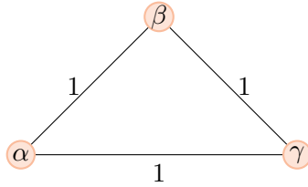
Figure 1: The graph representing the data vector \mathbf{v}_{\alpha\beta\gamma} .
