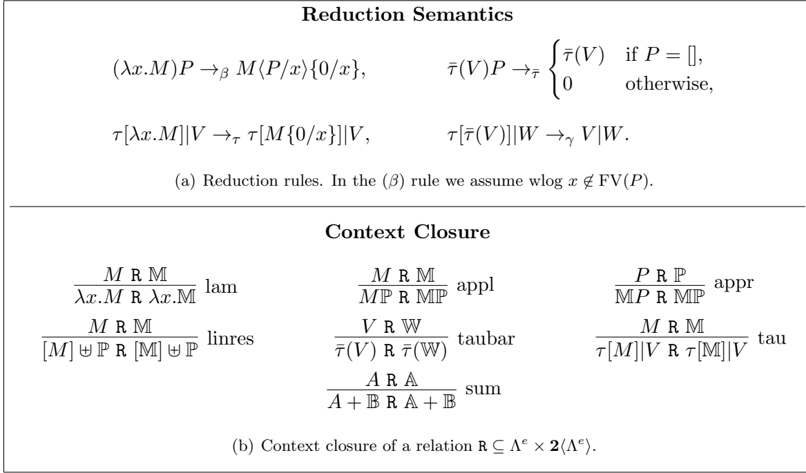
Figure 3: Operational Semantics.
