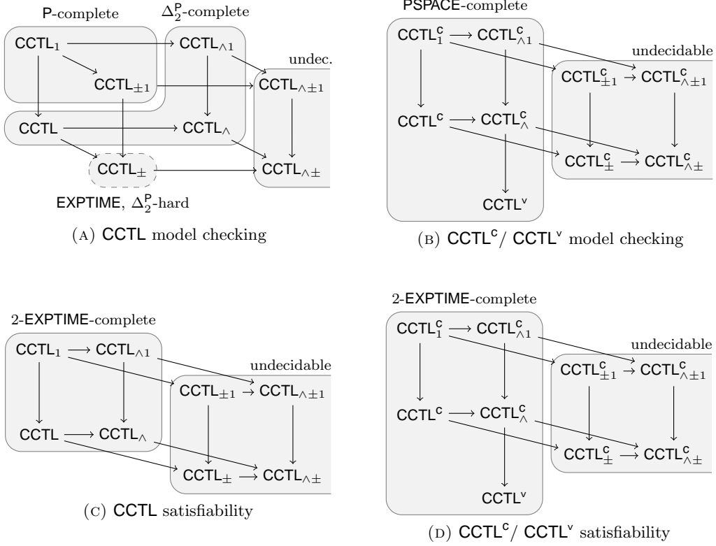
FIGURE 3. Summary of model-checking and satisfiability complexity results. Arrows indicate syntactic inclusion or straight-forward linear translations (case of CTL v ).
