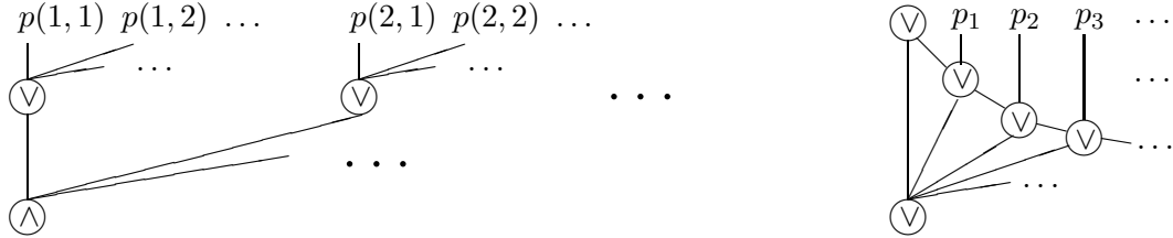
Figure 2: Infinite cirquents
