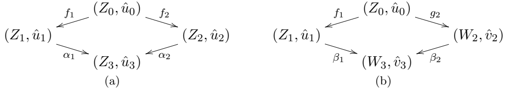
Figure 6: Pushouts in ONet .
