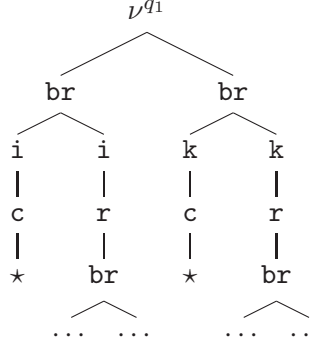
Figure 2: The tree generated by the recursion scheme of Example 5.5
