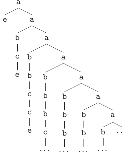
Figure 1: The tree generated by the recursion scheme of Example 1
