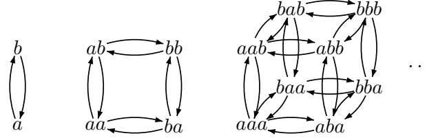
Figure 1: A finite portion of the relation \rightarrow from Example 3.2 extended to \{a, b\}^+ .
