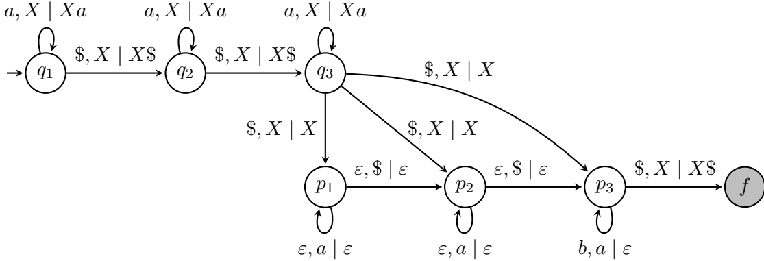
Figure 5: The PDA \mathcal{P}_{B_3} for B_3 . Grey states are final, and X is an arbitrary stack symbol.
