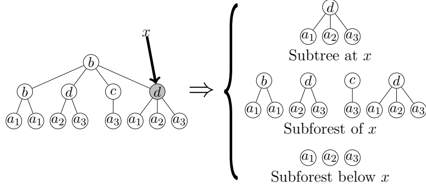
Figure 2: Illustration of the notion of subtrees and subforests
