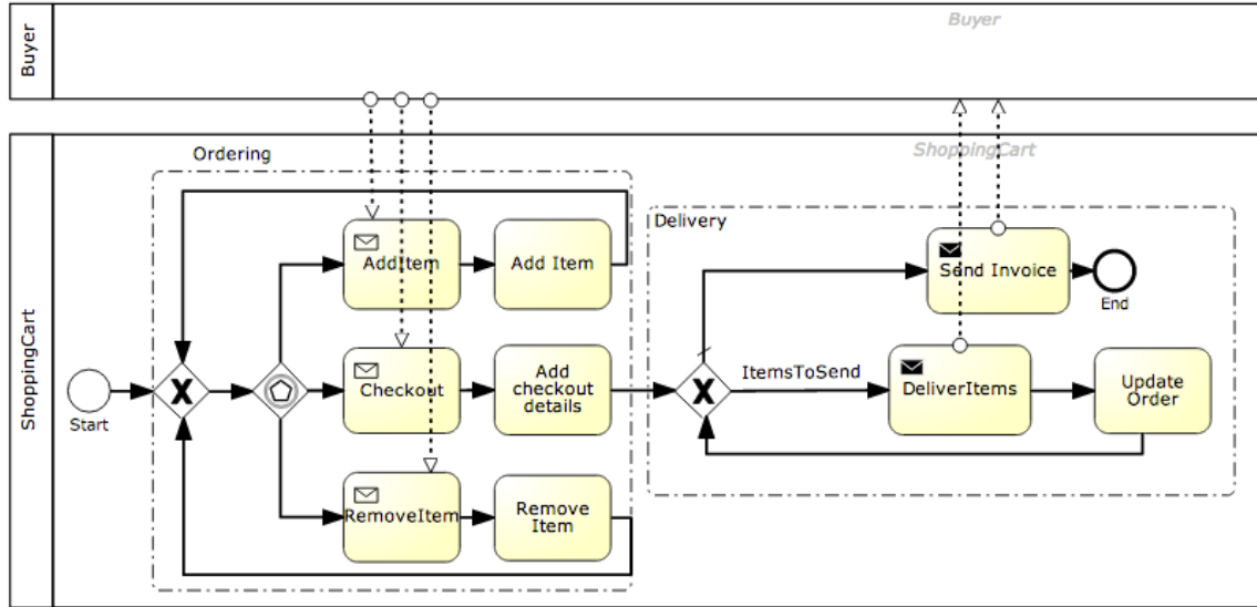
Figure A: A Potentially Non-live Shopping Cart BPMN Process
