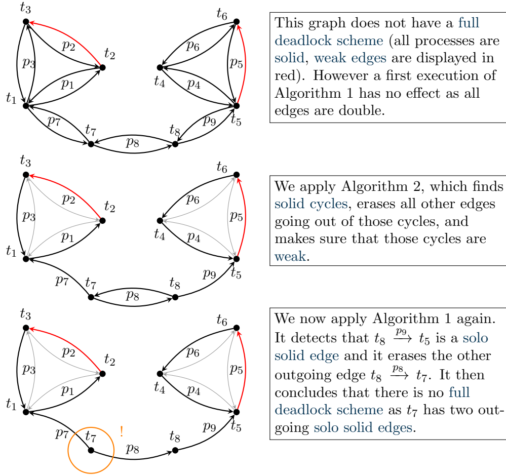
Figure 4: An example of application of Algorithm 2.
