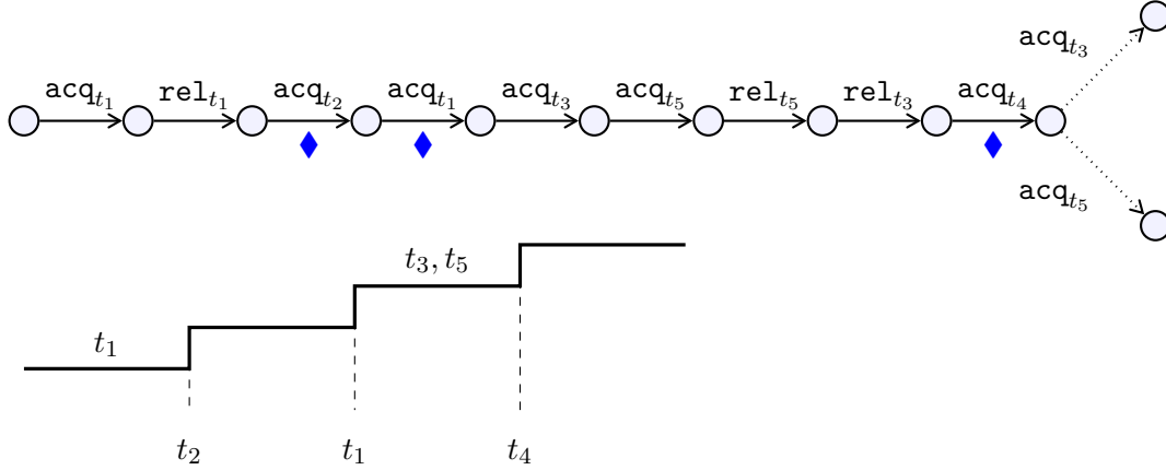
Figure 7: Example of a nested-locking local run. The dotted arrows are the available transitions at the end of the run. Blue diamonds mark transitions taking a lock that is not released later in the run. The lower part shows the stair pattern of this run (without the Blocks part). Steps represents the points at which a lock is taken and not released later. On each step we write the set of locks used in the corresponding section of the run.
