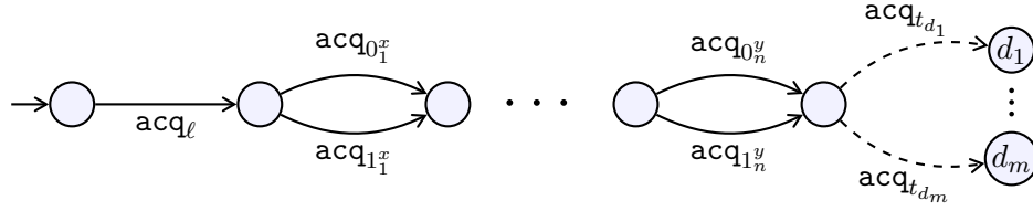
Figure 8: Transition system for process p for the proof of Theorem 2.13 (with D = \{d_1, \dots, d_m\} ). Dashed arrows are controlled by the system.
