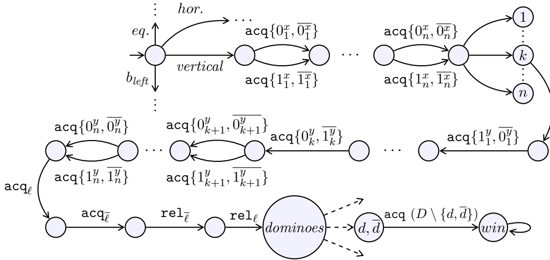
Figure 9: Transition system for process q in the proof of Theorem 2.13. Dashed arrows are controllable, every state before dominoes has a self-loop (not drawn) and \text{acq } S means a sequence of forced transitions with the operations \text{acq}_{t_i} for each t_i \in S (in some order). For simplicity only the vertical case is shown.
