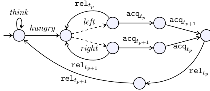
Figure 2: A flexible philosopher p . She can release a fork if the other fork is not available.
