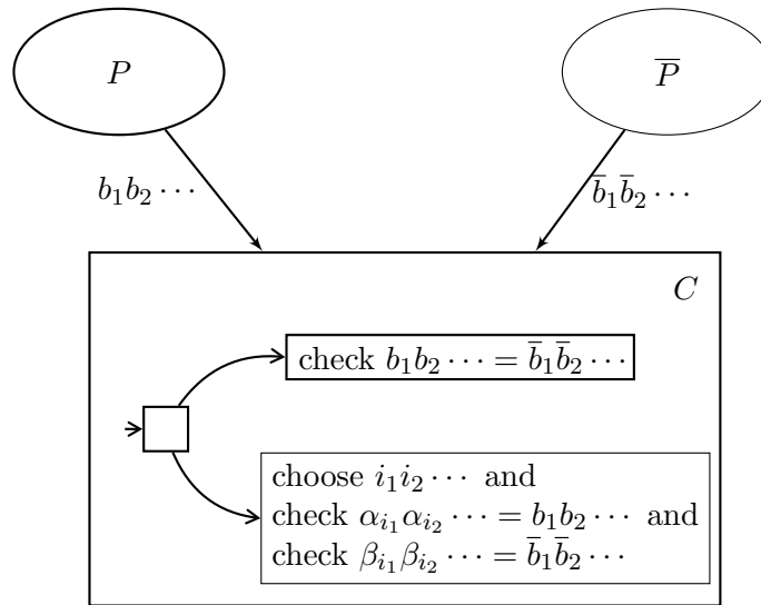
Figure 10: High-level view of the undecidability proof.
