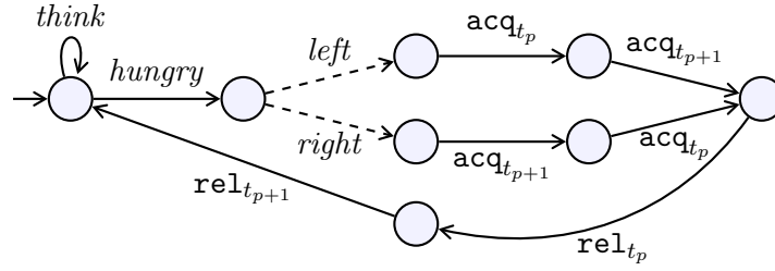
Figure 1: A dining philosopher p . Dashed transitions are controllable .
