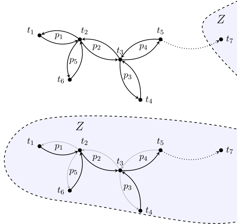
Figure 5: Illustration of Algorithm 3. A deadlock in Z can be extended to all these processes by orienting all edges/processes towards Z (black arrows in the bottom part).
