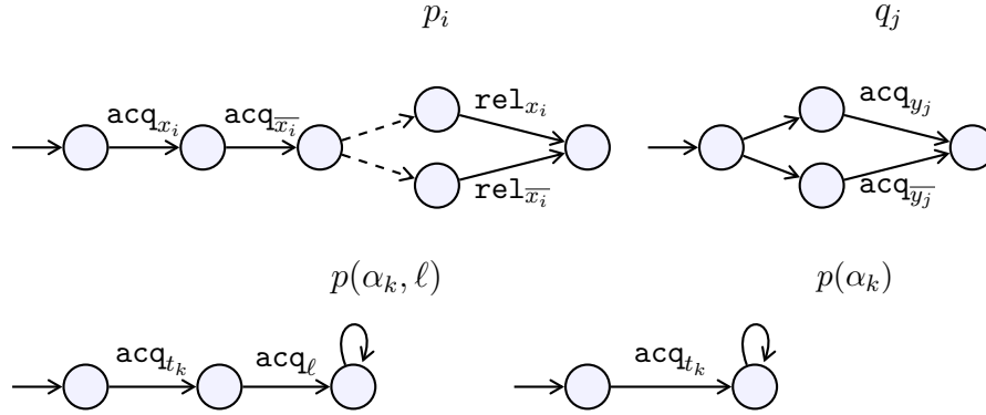
Figure 3: Processes used in Theorem 2.7. Transitions of the system are dashed. All unlabeled transitions carry nop as operation. Processes p_i and q_j handle existentially and universally quantified variables, resp.; process p(\alpha_k, \ell) handles literal \ell in clause \alpha_k , and process p(\alpha_k) handles clause \alpha_k .
