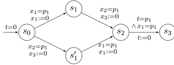
Figure 8: Encoding 0-test over bounded-time
