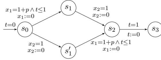
Figure 5: Encoding incrementation with a rational parameter
