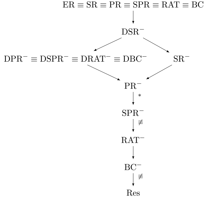
Figure 1: Relationships between proof systems.
