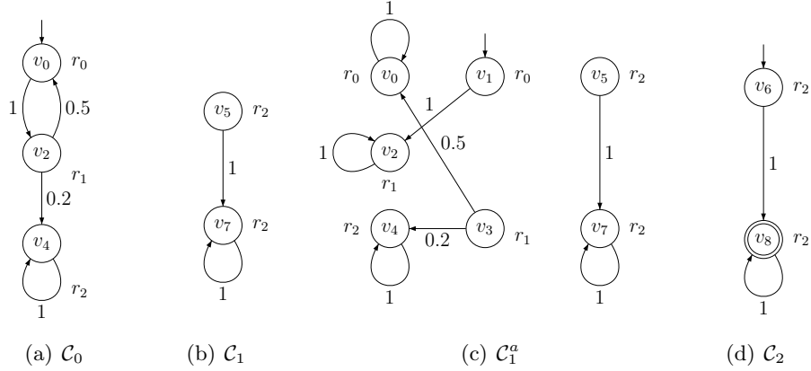
Figure 10: CTMCs corresponding to the (augmented) subgraphs
