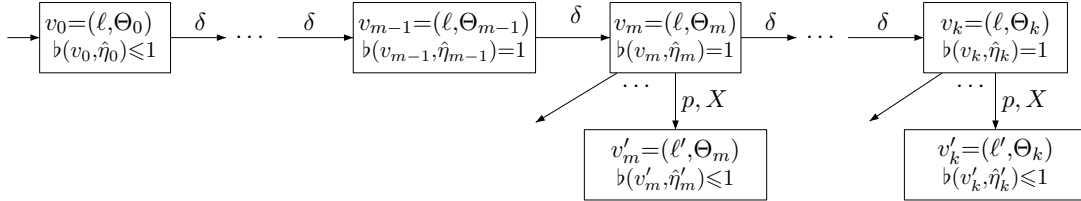
Figure 8: The sub-region graph \mathcal{Z}(\mathcal{C} \otimes \mathcal{A}) for the transition from \ell to \ell' .
