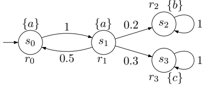
(b) CTMC \mathcal{C}
