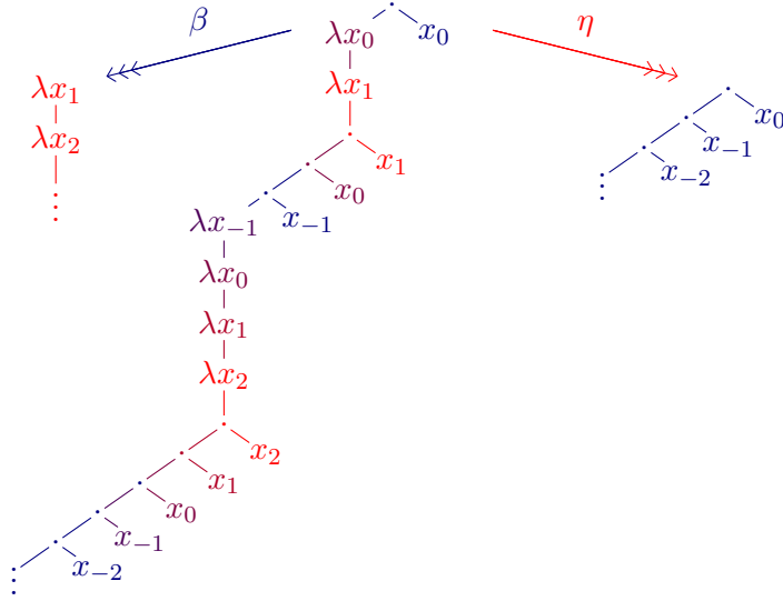
Figure 3: Counterexample to unique normal forms in \lambda^\infty\beta\eta .
