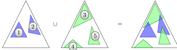
Figure 10: Orthogonalization in a weakly orthogonal TRS.
