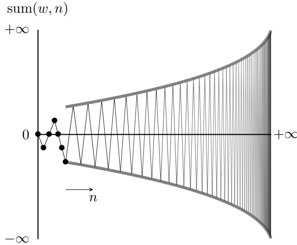
Figure 1: Graph for the oscillating PS -word \psi = P^1 S^2 P^3 \dots .
