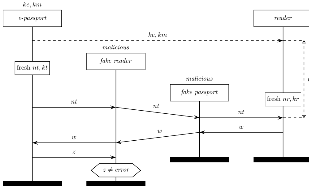
Figure 11: Message sequence chart representation of the left branch in Fig. 10 for \text{System}_{BAC} .
