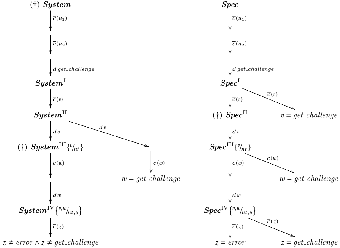
Figure 8: Distinguishing strategy implied by distinguishing formula \psi .
