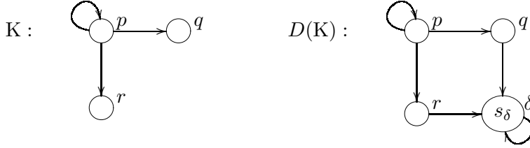
Figure 5: Deadlock extension of a Kripke structure
