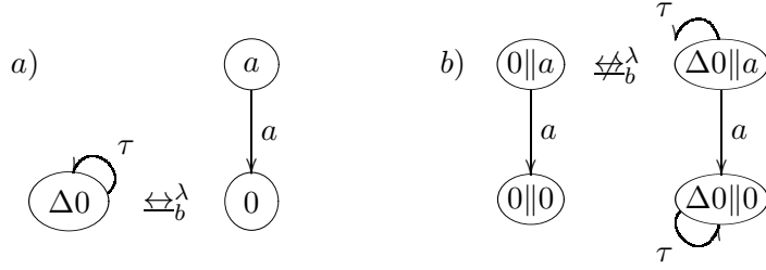
Figure 4: \u2194_b^\lambda is not a congruence for parallel composition
