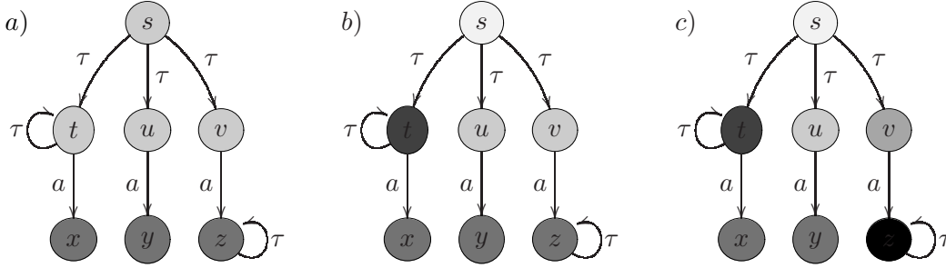
Figure 2: Difference between a) \stackrel{\Delta}{\leftrightarrow}_b , b) \stackrel{\lambda}{\leftrightarrow}_b , and c) \stackrel{\Delta}{\leftrightarrow}_b .
