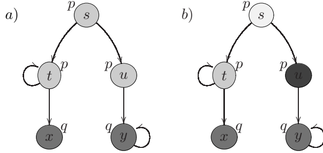
Figure 1: Difference between a) \approx_{db_s} and b) \approx_s .
