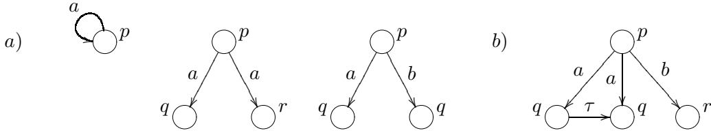
Figure 3: a) Three inconsistent L^2TS s and b) a consistent L^2TS .
